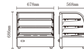
HW-120
