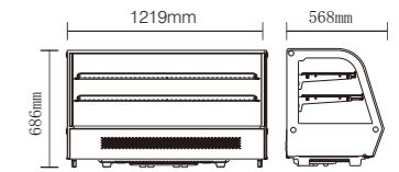
CW-200
