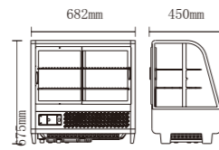
CW-100
