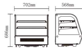
CW-120
