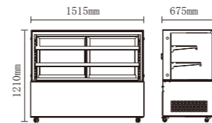
CW-470
