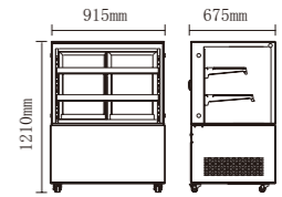
CW-270
